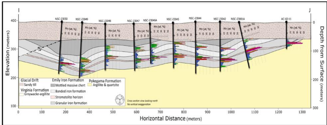
Figure 2. 2023 Drill Program – East to West Cross Section
