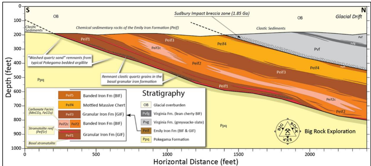
Figure 3. Emily Deposit – Schematic Stratigraphic Profile
